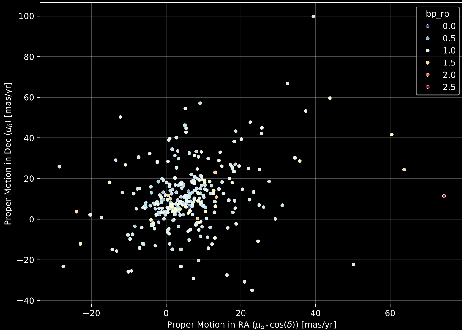
GALAH DR4 Field: [475] Proper Motion Diagram (n= 298)
