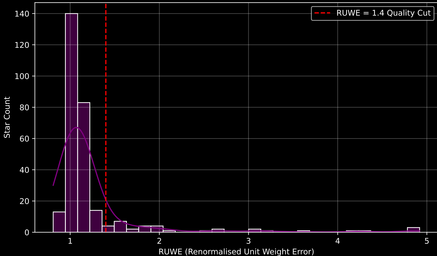
GALAH DR4 Field [475] RUWE Distribution (n= 284)
