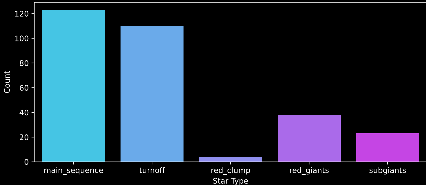
GALAH DR4 Field: [475] Count plot of Star Type
