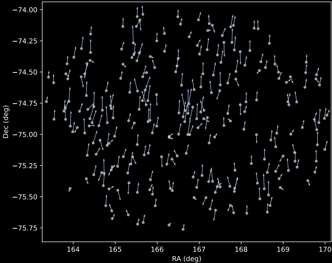
GALAH DR4 Cluster 1 Proper Motion Vectors (n=252)
